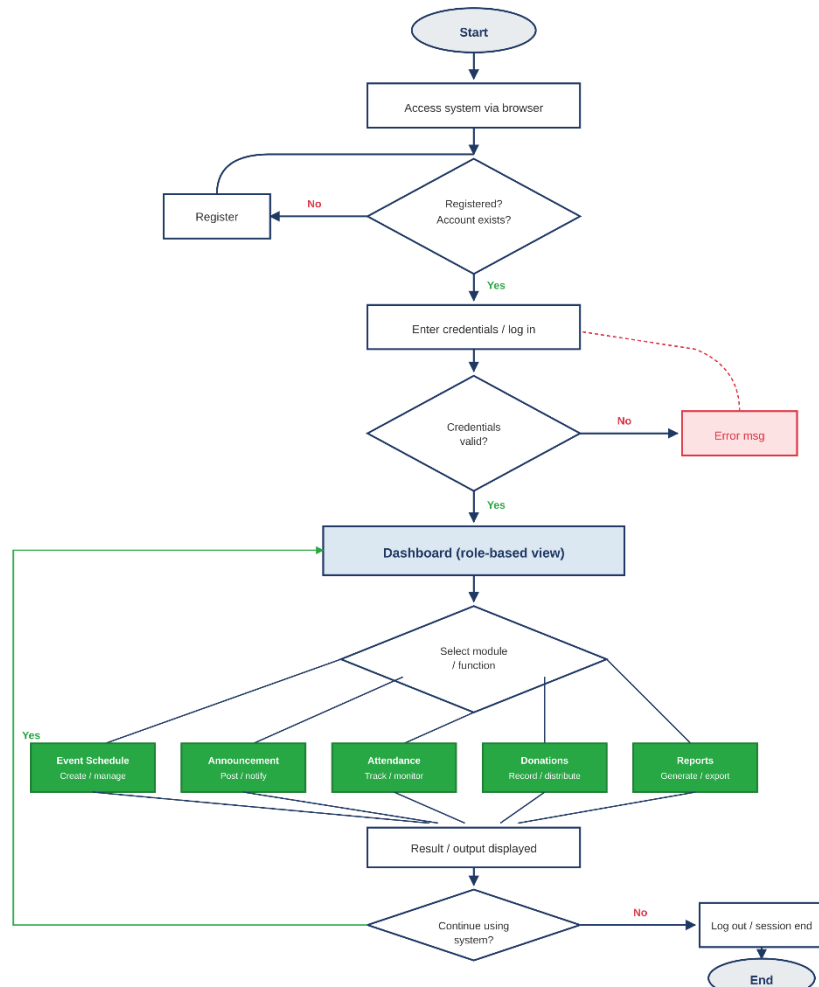
Figure 5. System Flowchart
